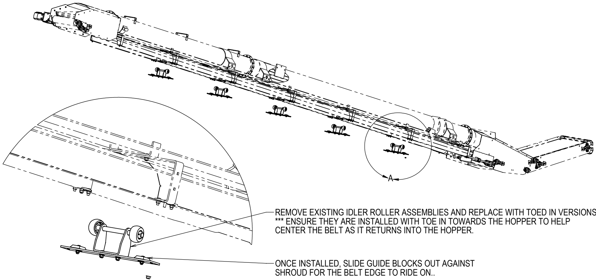
DETAIL A SCALE 1 : 10
