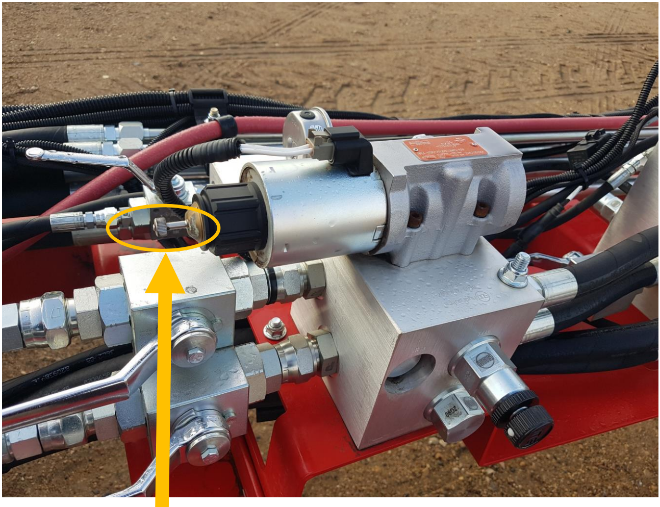
Manual Override Screw
