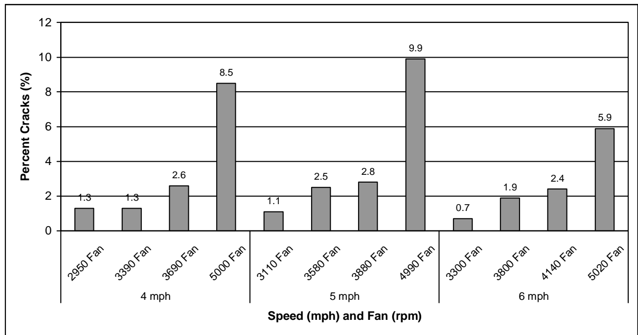
Figure 1. Effect of the Bourgault Ground and Fan Speed on Chickpea Damage.
